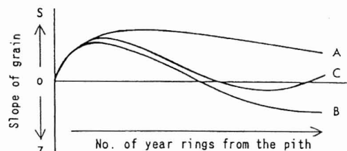
図-35 回旋角の樹幹半径方向における変動タイプ An illustration of radial variation types of slope of grain(OZAWA 1984).
