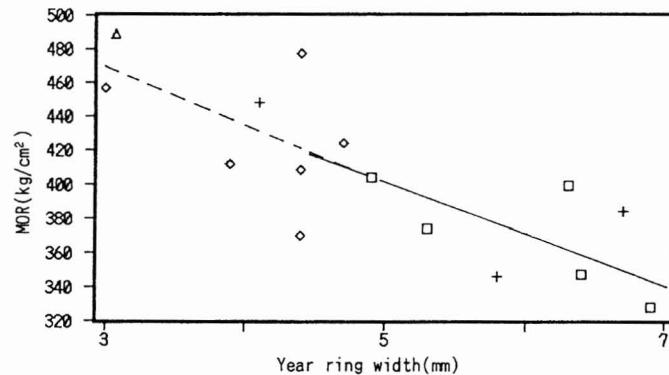
図-52 北海道、長野別カラマツ林分での年輪幅と曲げ強度との関係 Relationship between year ring width and bending strength(MOR) of sampled stands in Nagano and Hokkaido. □+: Hokkaido, ◇△: Nagano
