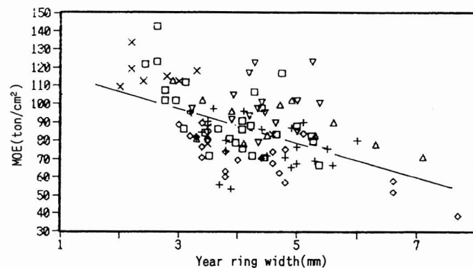
図-49 長野の林分における心持正角材の年輪幅と曲げヤング係数との関係 Relationship between year ring width and modulus of elasticity in bending(MOE) of sampled specimens in Nagano. □:Kurohime, +:Inekoki, ◇:Hase, △:Kitaiki, ×:Usuda, ▽:Motizuki.
