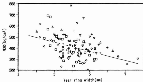
図-53 長野の林分における心持正角材の年輪幅と曲げ強度との関係 Relationship between year ring width and bending strength(MOR) of sampled specimens in Nagano. □:Kurohime, +:Inekoki, ◇:Hase, △:Kittaiki, ×:Usuda, ▽:Motizuki.
